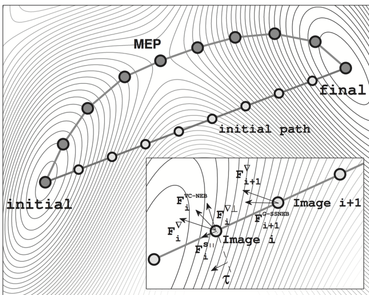
Figure 15: The minimum energy path (line with gray circles) and initial path on a model 2D enthalpy surface. The forces in the VCNEB method on image i are shown in the inset. F_i^{\nabla} is the potential force in the gradient direction. F_i^{\nabla\perp} and F_i^{s\parallel} are the transverse component of F_i^{\nabla} and the spring force, respectively.
