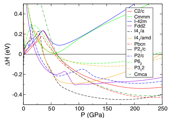
FIG. 2 (color online). Enthalpies of the most favorable structures. Interestingly, at 55 GPa, four competing structures have the same enthalpy and silane changes from intermediate between molecular and polymeric to a fully polymeric phase. The P6_3 structure lies always at least 1 eV above the reference P2_1/c structure. Lines are only a guide to the eye, the actual enthalpies being calculated at discrete intervals.
