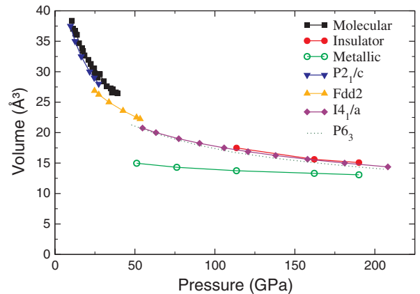
FIG. 3 (color online). Theoretical equation of state (EOS) of silane, compared with the experimental one [16]. Also included is the equation of state corresponding to the relaxed P6_3 structure. Note the discrepancy between the EOS of metallic silane and the calculations for all other phases.
