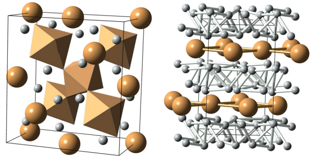
FIG. 1 (color online). Novel structures of silane. Large atoms depict Si, while small atoms represent H. Left: Fdd2 silane, stable between 25 and 55 GPa. Right: Pbcn silane, which is metallic, superconducting and favored above 220 GPa.
