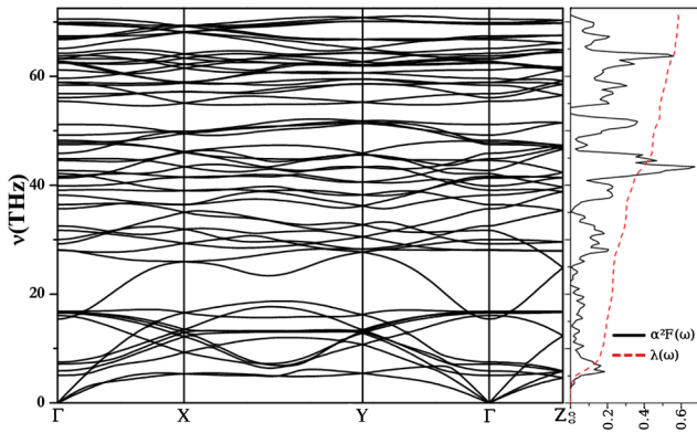
FIG. 4 (color online). Phonon dispersion and spectral Eliashberg function of the Pbcn structure at 190 GPa. This pressure has been chosen to show a better comparison to experiment [16]. At 190 GPa, Pbcn silane has a T_c = 16.5 K, in nice agreement with the experimental value ( T_c = 12 K).
